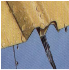
Rainguard Side Lap Drain Channel Prevents Capillary Siphon Action
