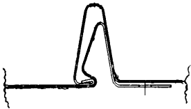
Seam Snapped Together
