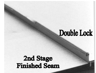
Double Lock Standing Seam 17-5/8"
